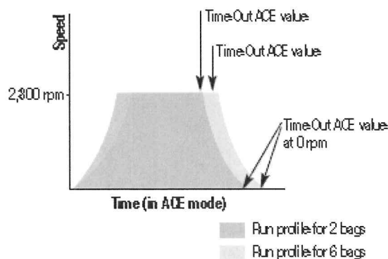
Figure 2: With an ACE value and speed set at the start of a run, times were adjusted to achieve the same overall g-force regardless of the rotor load.
