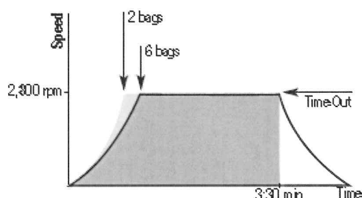
Figure 1: In a typical first centrifugation step, a two-bag rotor load attains set speed faster than a six-bag load. Since both loads will time out at the set time of 3:30 minutes, different g-forces are achieved during the run. By using the ACE integrator function, the time for 2 bags would be changed to 3:00 minutes to obtain the same overall g-force for both loads.
